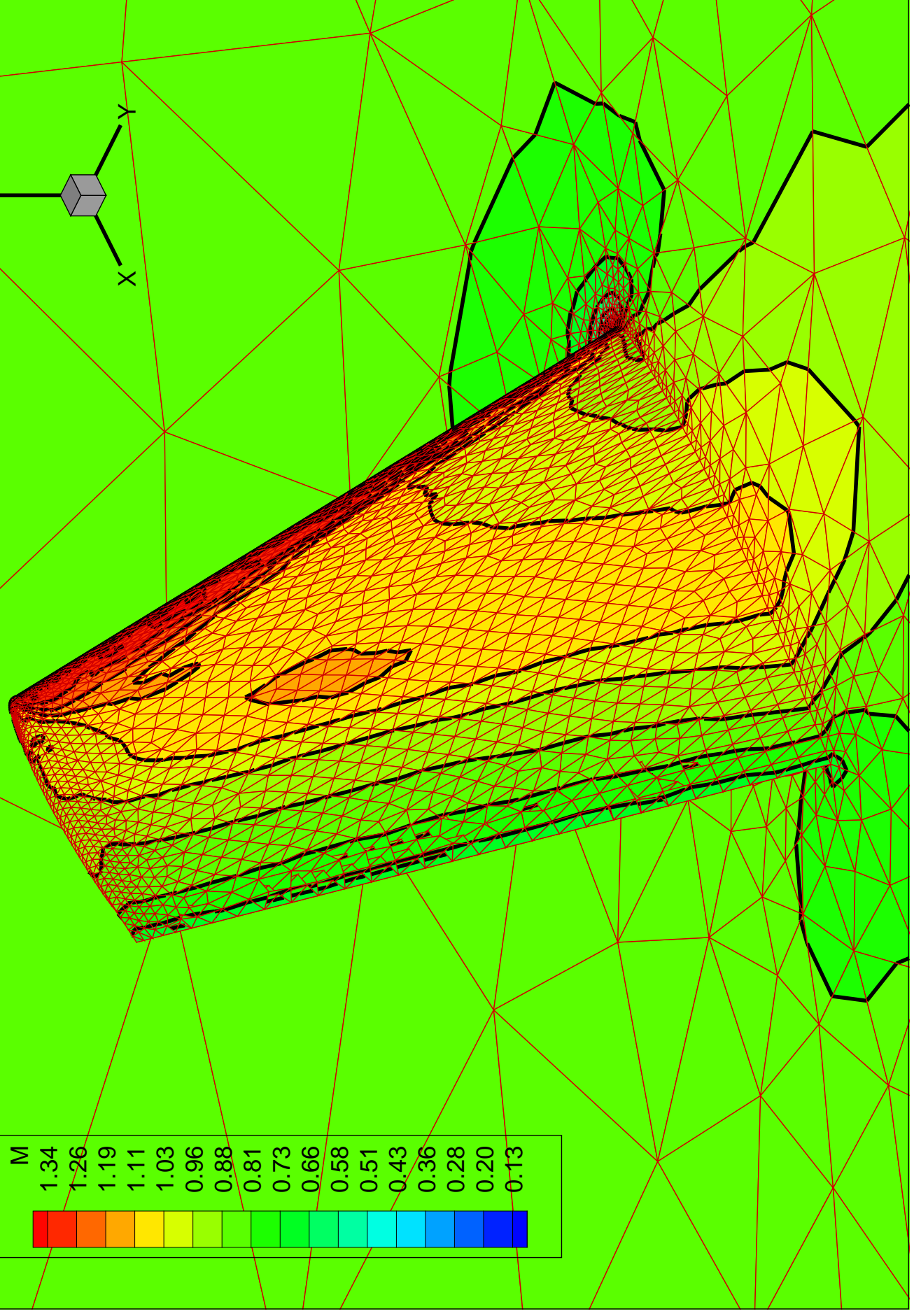
Mach contours on surface of ONERA M6 wing ( \alpha = 3.06^\circ , M = 0.84 )
