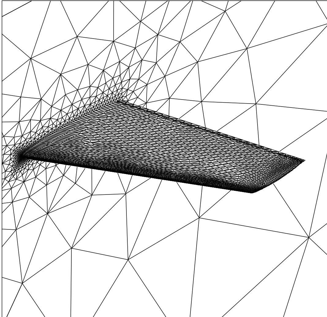
Surface grid and nearfield symmetry plane.
